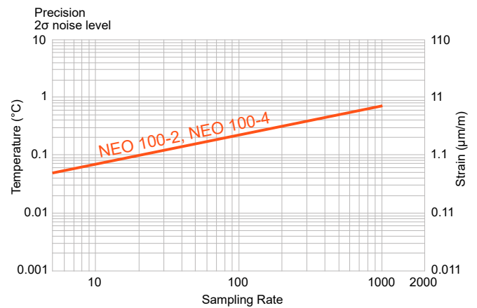
Typ Precision vs. Sampling Rate (Hz)
