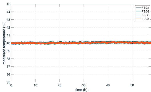
Long-Term Stability (<0.06 °C @ 60 h, \sigma )
